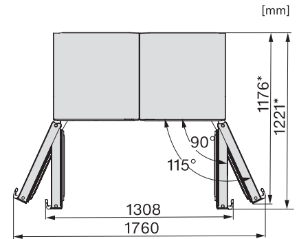
KS4383ED N, KS4384ED N, FNS4382E N, FNS4383E N, Nordic, top view, Side-by-Side (*footnote) (installation drawings)
