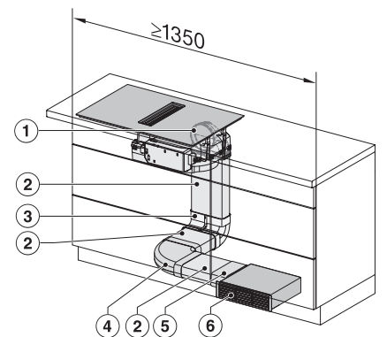
KMDA7676FL, KMDA7876FL – Installation variant 1 Basis -drawing
